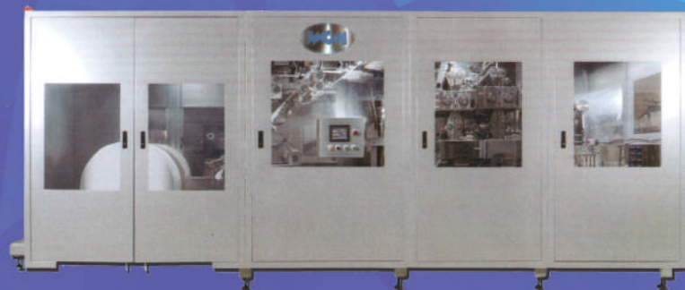
W-120 全自動濕巾包裝機 8片-10片裝 Fully Auto Wet Tissue(8'-10's) Packing Machine FWP-300 全自動濕巾單片包 Wet Tissue Packing Machine
